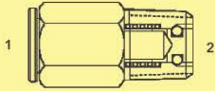
BPC-SO-2404 - Str. (1) Tube (2) Male Pipe w/Shut Off Valve
