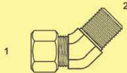
BC-2503 - 45° (1) Compression (2) Male Pipe
