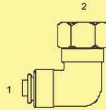
BPC-DOT-2502-S - 90° (1) Tube (2) Fem. Pipe Swivel
