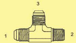
BJ-2605 - Tee (1) (3) Male 37° (2) Male Pipe
