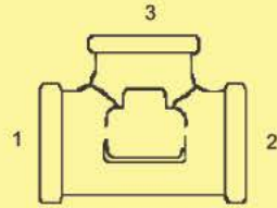
BP-5605-F - Tee (Forged) (1) (2) (3) Fem. Pipe
