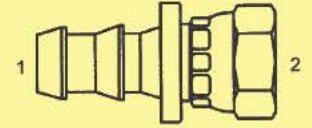
BPO-2280 - Str. (1) Hose Barb (2) Fem. Pipe Swivel Gasket Seat
