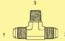
BJ-2601 - Tee (1) (2) Male 37° (3) Male Pipe
