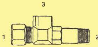
BC-2611 - Tee (1) Compression (2) Male Pipe (3) Fem. Pipe
