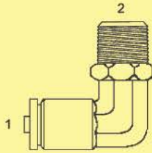
BPC-DOT-2501-S - 90° (1) Tube (2) Male Pipe Swivel
