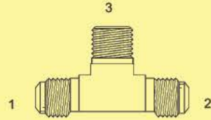
BF-2601 - Tee (1) (2) Male 45° (3) Male Pipe
