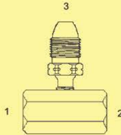
B-POL-2001 - Tee Manifold Block Tee Assembly (1) (2) Fem. POL (3) Male POL
