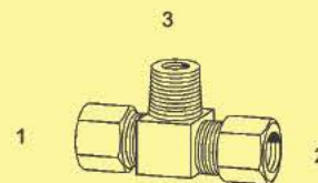
BC-SA-2601 - Tee (1) (2) Compression (3) Male Pipe
