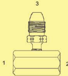
B-POL-2001-CV - Tee Manifold Block Tee Assembly with Check Valve (1) (2) Fem. POL (3) Male POL
