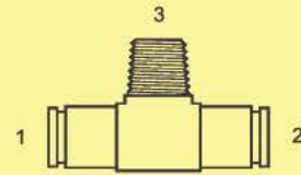
BPC-NI-2601 - Tee (1) (2) Tube (3) Male Pipe
