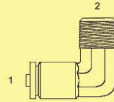
BPC-DOT-2501 - 90° (1) Tube (2) Male Pipe
