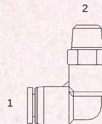
CPC-SB-2501-S - 90° (1) Tube (2) Male Pipe Swivel
