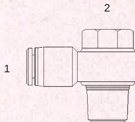
CPC-4110 - Banjo
