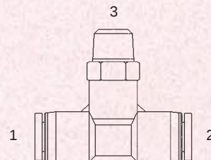
CPC-SB-2601-S - Tee (1) (2) Tube (3) Male Pipe Swivel
