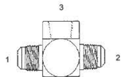
2602 - Tee (1) (2) Male Tube (3) Female Pipe
