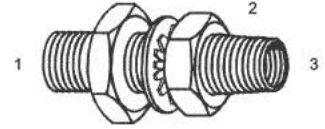
5404-BH - Str. (1) (2) Male Pipe (3) Fem. Pipe 1/4"
