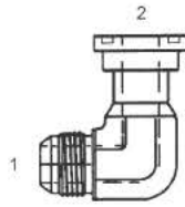
1704-F-62 - 90° Forged (1) Male 37° (2) O Ring Flange Code 62
