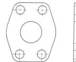
SF-62-CP Connector Plate Code 62
