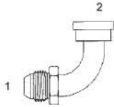
1704-62 - 90° (1) Male Tube (2) O Ring Flange Code 62
