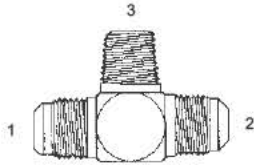
2601 - Tee (1) (2) Male Tube (3) Male Pipe
