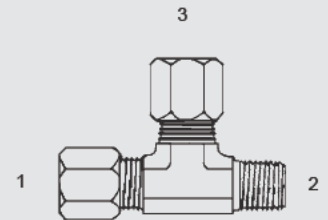
Y-FL-2605 - Tee (1) (3) Male Flareless (2) Male Pipe
