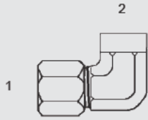
Y-FL-2502 - 90° (1) Male Flareless (2) Fem. Pipe
