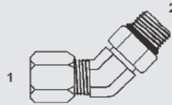
Y-FL-6802- NWO - 45° (1) Male Flareless (2) Adj. O-Ring
