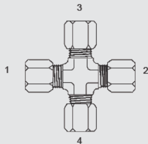
Y-FL-2650 - Cross
