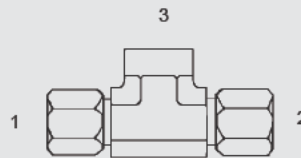
Y-FL-2602 - Tee (1) (2) Male Flareless (3) Fem. Pipe
