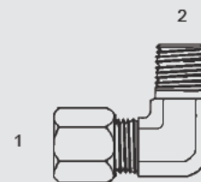
Y-FL-2501 - 90° (1) Male Flareless (2) Male Pipe
