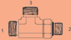
Y-OFS-6804-F-NWO - Tee (1) (3) Male OFS (2) Adj. O-Ring
