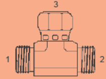
Y-OFS-6600-F - Tee (1) (2) Male OFS (3) Fem. OFS Swivel
