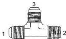
Y-2605-F - Tee (1) (3) Male 37° (2) Male Pipe
