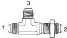
Y-2704-F-LN - Tee (1) (3) Male 37° (2) Bulkhead 37° w/ Locknut
