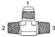
Y-2610-F - Tee (1) Male 37° (2) (3) Male Pipe
