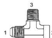
Y-2608-F - Tee (1) Male 37° (2) Fem. Pipe (3) Male Pipe
