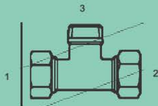
MFL-MT-2601 - Tee (1) (2) Male Flareless (3) Male Metric Taper Light
