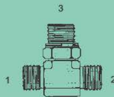
BPP-OFS-6803-NWO - Tee (1) (2) Male O Ring Face Seal (SAE) (3) Male BPP Adj. O Ring w/ Retainer Washer
