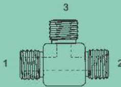
BPP-5600 - Tee (1) (2) (3) Male BPP
