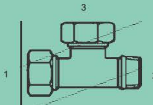
MFL-MT-2605 - Tee (1) (3) Male Flareless (2) Male Metric Taper Light
