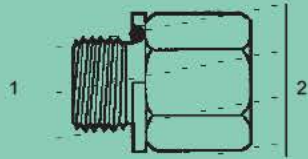
M-FP-6405-DS - Str. (1) Male Metric w/ Bonded Seal (2) Fem. NPT Pipe
