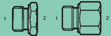
M-6410 - Str. (1) Male Metric (Parallel) (2) Fem. Metric (Parallel) (Length of Hex may vary)
