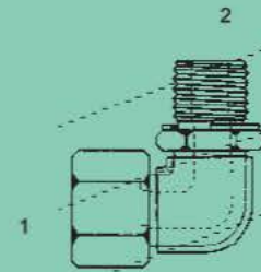
MFL-M-6801-NWO - 90° (1) Male Flareless (2) Male Metric w/ Washer O Ring Light
