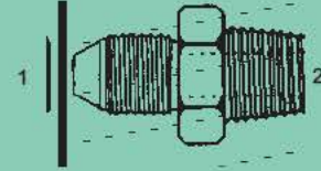
JISBP-MP-2404 - Str. (1) Male 30° BPP (Flare) (2) Male NPT Pipe
