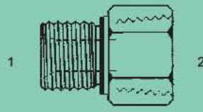
M-FP-6405-WO - Str. (1) Male Metric w/ Washer & O Ring (2) Fem. NPT Pipe
