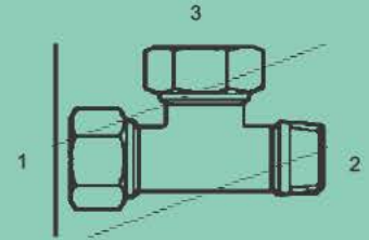
MFL-MT-2605-H - Tee (1) (3) Male Flareless (2) Male Metric Taper Heavy
