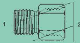
BPP-FB-6410 - Str. (1) Male BPP (2) Fem. O Ring
