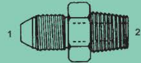
JISM-MP-2404 - Str. (1) Male 30° Metric Komatsu (2) Male NPT Pipe
