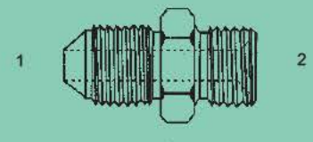
M-MJ-2404 - Str. (1) Male 37° (2) Male Metric (Parallel) (Some w/ 30° seat and some w/ 24° seat)
