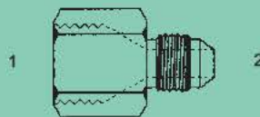
JISM-MJ-2406 - Str. (1) Fem. 30° Metric Komatsu (2) Male 37°
