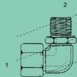
MFL-M-6801-H-NWO - 90° (1) Male Flareless (2) Male Metric w/ Washer O Ring Heavy
