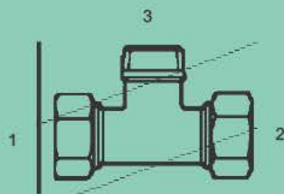
MFL-MT-2601-LL - Tee (1) (2) Male Flareless (3) Male Metric Taper Extra Light
