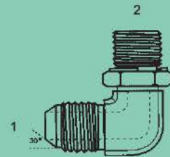
JISBP-BPP-6801-NWO - 90° (1) Male 30° BPP (Flare) (2) Male BPP Adj. O Ring
