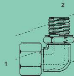
MFL-M-6801-NWO-ISO - 90° (1) Male Flareless (2) Male Metric w/ ISO O Ring 6149
