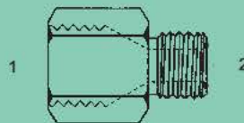
JISBP-MOFS-2406 - Str. (1) Fem. 30° BPP (Flare) (2) Male O Ring Face Seal (SAE)
