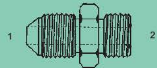
JISM-OFS-2403 - Str. (1) Male 30° Metric Komatsu (2) Male O Ring Face Seal (SAE)
