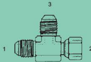
JISM-6602 - Tee (1) (3) Male 30° Metric Komatsu (2) Fem. 30° Metric Komatsu Swivel
