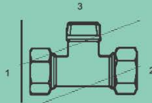
MFL-MT-2601-H - Tee (1) (2) Male Flareless (3) Male Metric Taper Heavy
