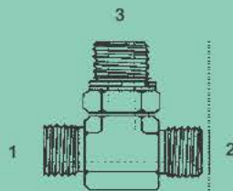
BPP-7803-NW0 - Tee (1) (2) Male BPP (3) Male BPP Adj. O Ring
