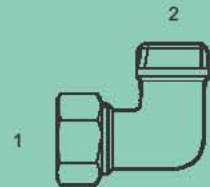
MFL-MP-2501-H - 90° (1) Male Flareless (2) Male NPT Heavy
