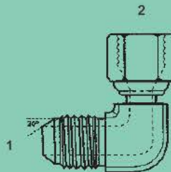
JISBP-6500 - 90° (1) Male 30° BPP (Flare) (2) Fem. 30° BPP (Flare) Swivel
