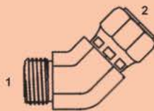
OFS-6502 - 45° (1) Male OFS (2) Fem. OFS Swivel
