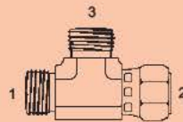
OFS-6602 - Tee (1) (3) Male OFS (2) Fem. OFS Swivel
