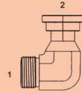
OFS-1704-F-62 - 90° Forged (1) Male OFS (2) O Ring Flange Code 62
