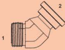
OFS-1703-F-61 - 45° Forged (1) Male OFS (2) O Ring Flange Code 61
