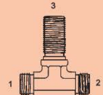
OFS-2703 - Tee (1) (2) Male OFS (3) OFS Bulkhead
