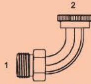
OFS-1704-61-H - 90° Heavy (1) Male OFS (2) O Ring Flange Code 61
