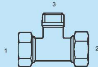
SS-MFL-MP-2601 - Tee (1) (2) Male Flareless (3) Male NPT
