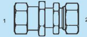
SS-MFL-2700-LN - Str. (1) Male Flareless (2) Male Flareless Bulkhead w/ Lock Nut Light
