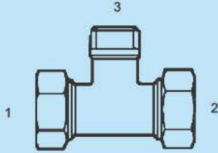
SS-MFL-MP-2601-H - Tee
