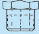
DIN 3852 Form C: Sealing by means of tapered thread. Female thread must be tapered to achieve rated operating pressure.
