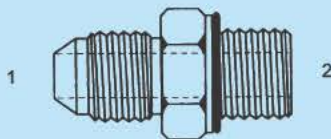
SS-M-MJ-6400-WO - Str. (1) Male 37° (2) Male Metric w/ Washer & O Ring
