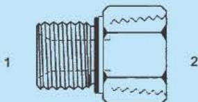
SS-M-FP-6405-WO - Str. (1) Male Metric w/ Washer & O Ring (2) Fem. NPT Pipe
