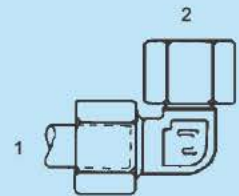
SS-MFL-6500-H - 90° (1) Male Flareless (2) Fem. Flareless Swivel Heavy
