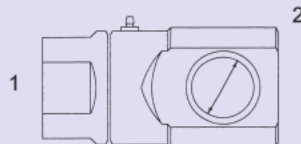
SLS-5504-SB - 90° (1) Fem. Pipe Stem (2) Fem. Pipe Barrel (Short Body)
