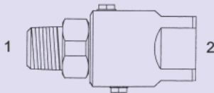
SLS-5405-HP - Str. High Pressure 10,000 PSI (1) Male Pipe Stem (2) Fem. Pipe Barrel
