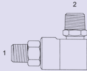
SLS-5500 - 90° (1) Male Pipe Stem (2) Male Pipe Barrel
